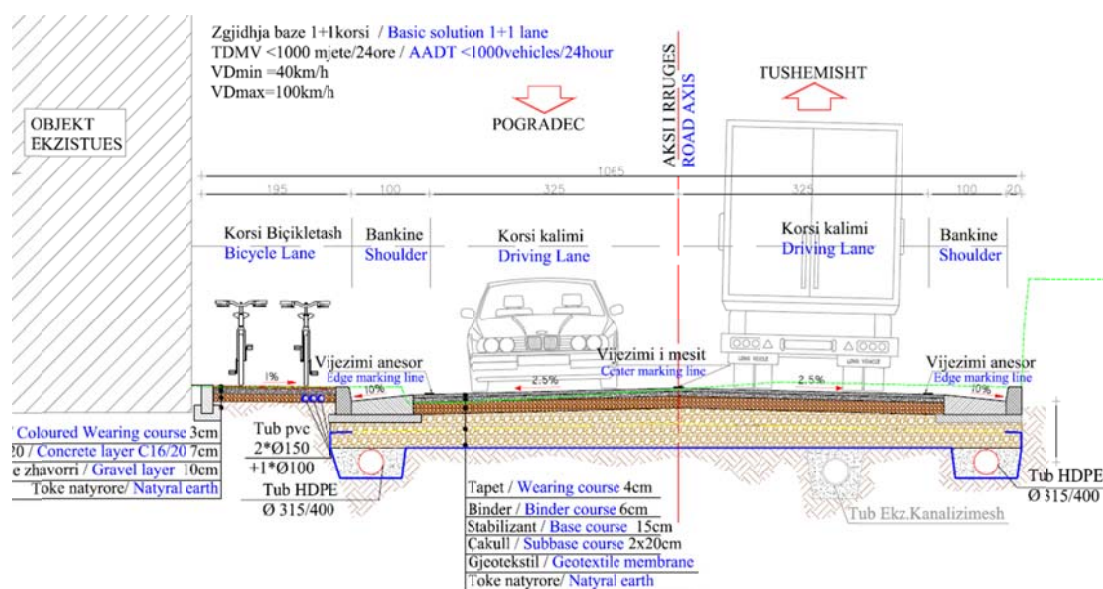
Figure 6: Existing infrastructure in urban parts of the road and proposed cross section
